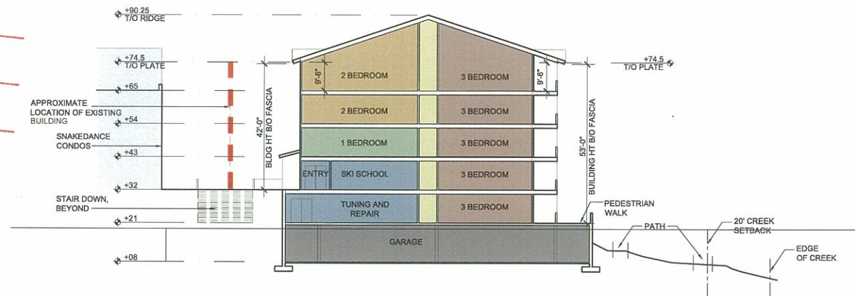
SECTION A
