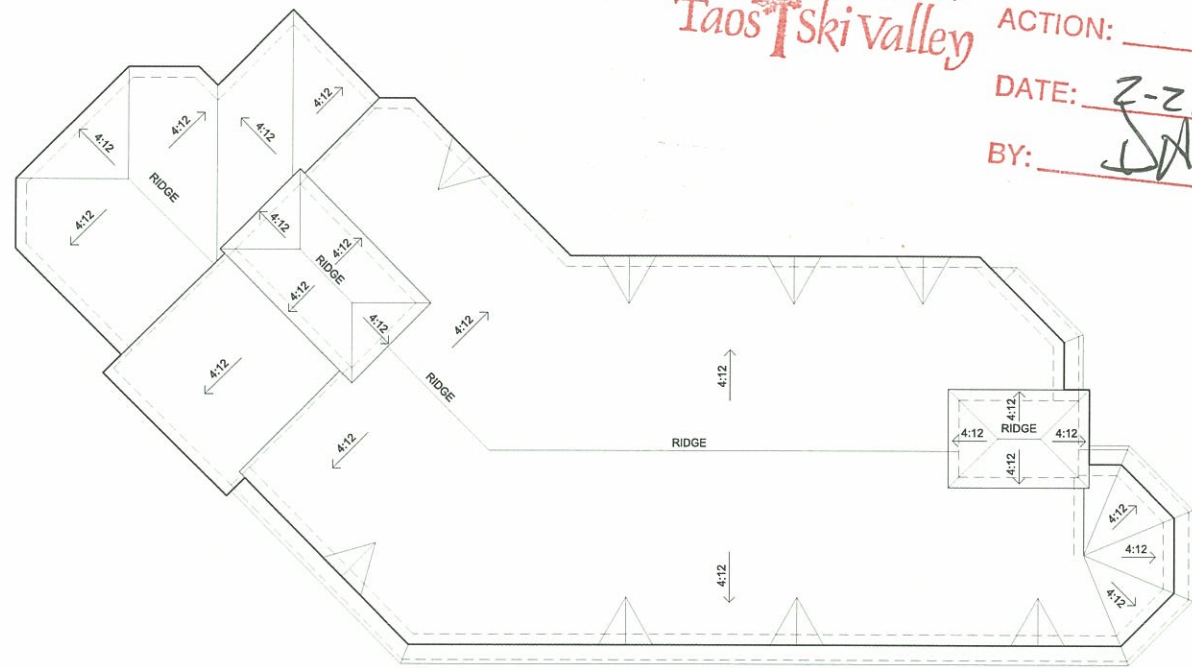
ROOF PLAN
