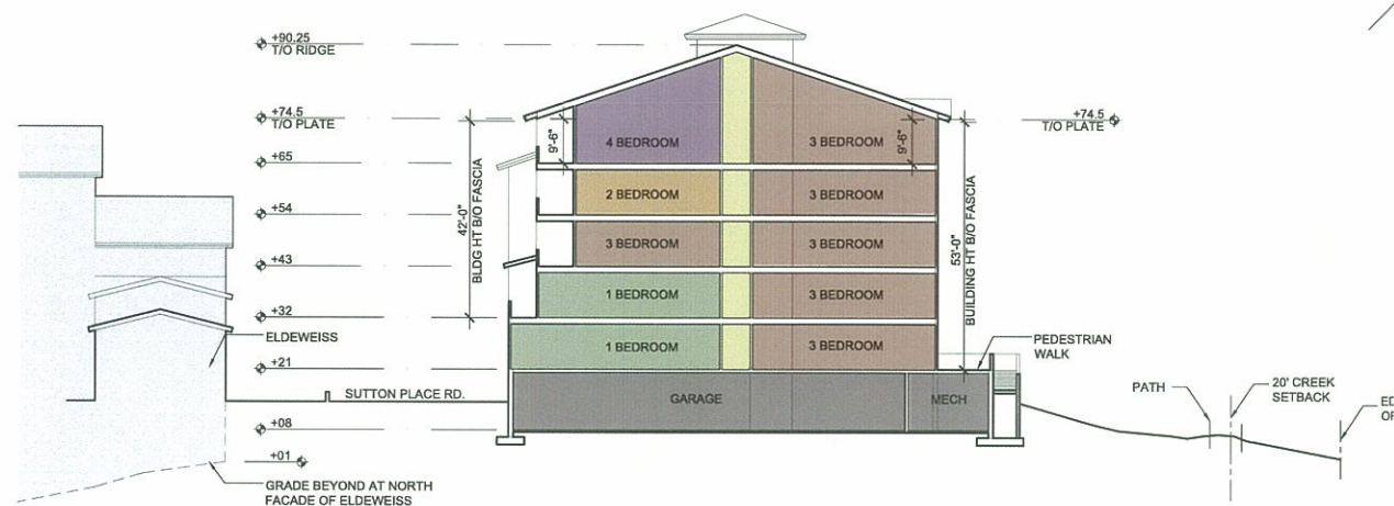
SECTION B
