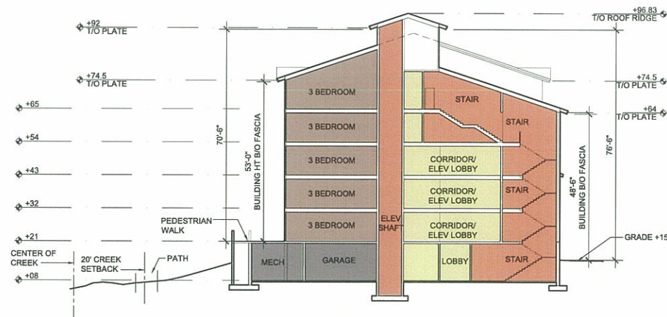
SECTION C
