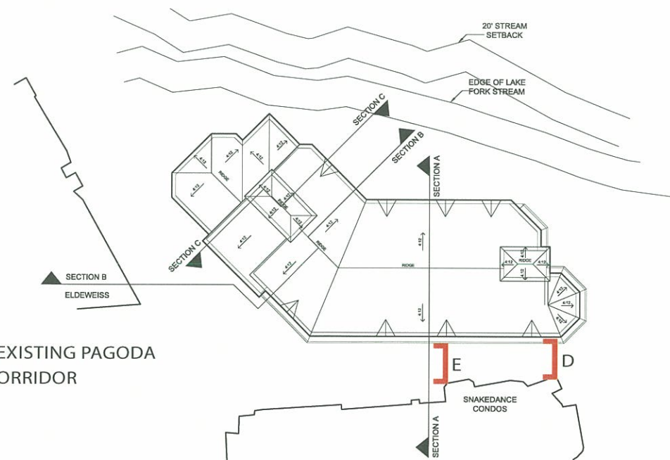
SECTION KEY
